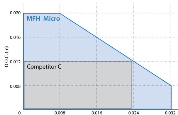
Cutting Performance Map (Cutter Dia. \emptyset 0.375 ")
