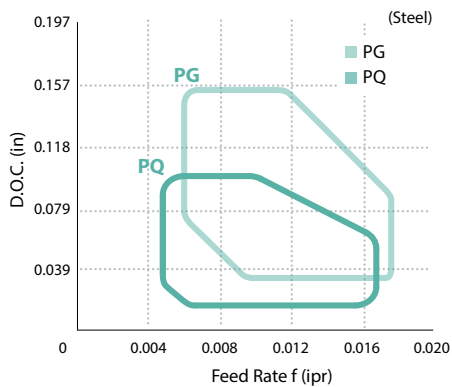
Chipbreaker Application Range
